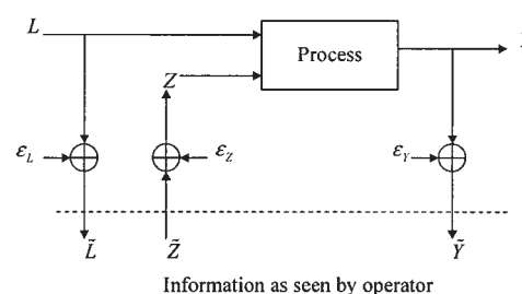
Figure 1. Schematic representation of measured quantities [as seen by an external operator and marked with a tilde ( \sim )] and the quantities that are actually involved in the underlying process.
